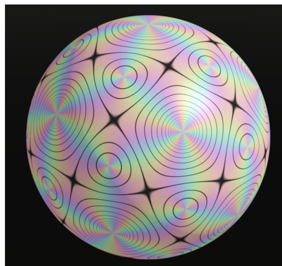
Klein’s icosahedral function drawn by Abdelaziz Nait Merzouk. The color shows its phase, while the contour lines show its magnitude
