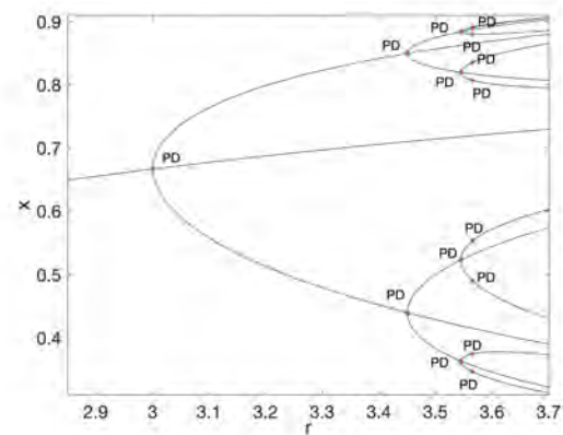
Figure 1. Re-creating the bifurcation structure of the logistic map using MatContM . PD denotes that the red stars are specifically period-doubling bifurcations.
