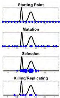
Figure 1. Sequential Monte Carlo
