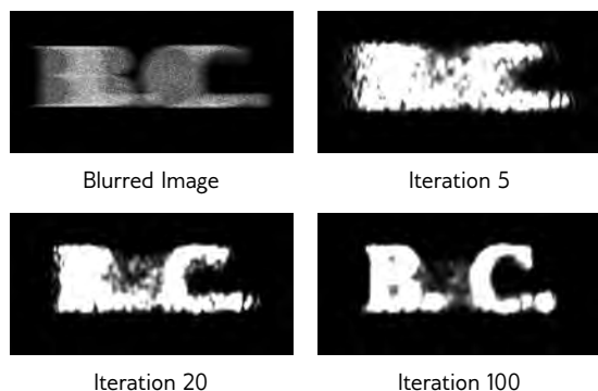
Figure 2. Given the blurred image, h , we iteratively reconstruct the original image, f . The function g describes the motion which caused the blur.
