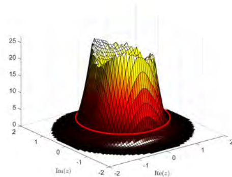
Figure 1. Random Fibonacci witch hat
