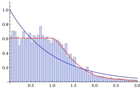
Figure 9. The gap distribution for the fractional parts of nu , with n = 1, \dots, 2000 and u sampled over 2000 randomly chosen points in [0, 1] . Theoretical curves are the exponential density e^{-s} (blue) vs. P(s) (red).
