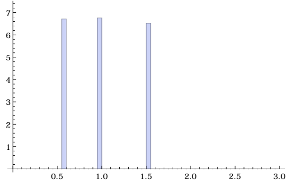
Figure 8. The gap distribution for the fractional parts of nu , with n = 1, \dots, 50000 and u = \pi .
